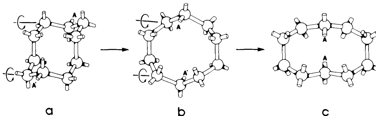
Figure 10. The deformation of the skeletal structure of cyclodecane into that of (\text{NPMe}_2)_{10} with a short central transannular distance, through an intermediate of symmetry D_{5d} .
