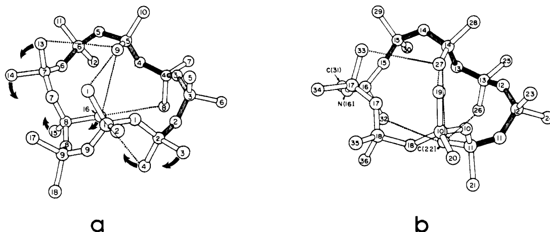
Figure 8. (\text{NPMe}_2)_9 : (a) molecule 1, (b) molecule 2. The common conformational fragment is shaded. Dotted lines join methyl groups separated by intraannular distances of 4.0 Å or less. The arrows show the movements required to convert molecule 1 to molecule 2.
