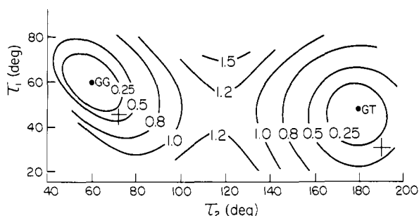
Figure 5. Local conformations (a-f) and potential energy (kcal/mol) of \text{Me}_2\text{P}(\text{NP})_2 fragment, using the parameters of ref 39 and average bond lengths and angles. \tau_1 and \tau_2 are measured from the cis-coplanar conformation d. The crosses are experimental points; see text.
