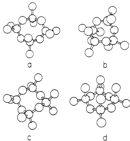
Figure 1. Symmetrical frameworks found in (ABX_2)_4 molecules; skeletal atoms shaded. (a) Chair, as in P_4O_{12}^{3-} and in (OSiMe_2)_4 . 4,5 (b) Tub, as in P_4O_{12}^{3-} and in (NPCI_2)_4 . 6,7 (c) Saddle, as in (NPM_2)_4 and in (OSeO_2)_4 . 8,9 (d) Crown, as in (NPCI_2)_4 and (with substituents on alternate atoms) in (NMe_2PMe)_4 . 10,11
