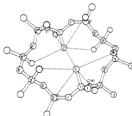
Figure 9. (\text{NPMe}_2)_{10} : Short intraannular Me...Me distances dotted. The axial methyl groups exhibit approximate pentagonal symmetry; one of two sets is shaded.
